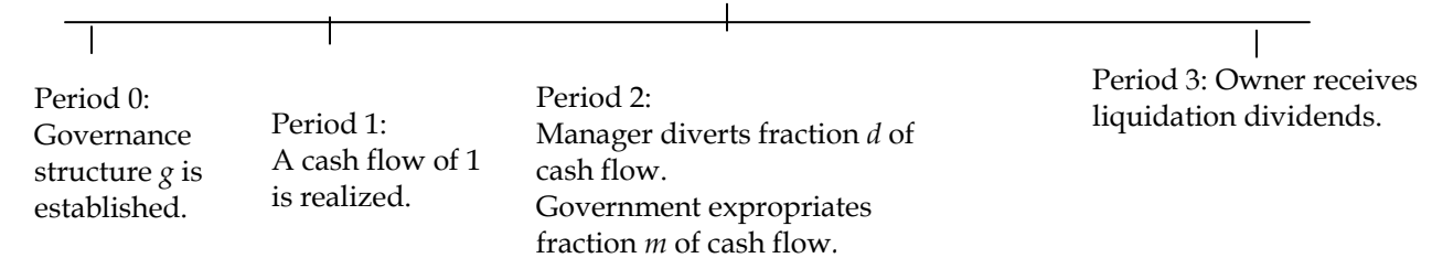
Figure 1: Model timing
