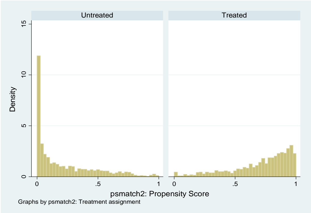
Figure A1: Support of Estimated Propensity Score by Treatment Status
