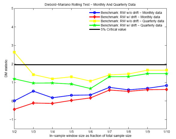
Panel II. Chilean Peso and Copper. Monthly and Quarterly Lagged Model
