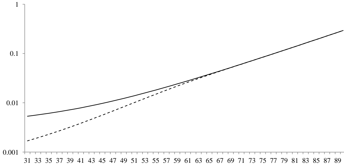
Figure 17: Simulated Mortality Rates 1871-79 for IBN people: Ages 30 to 90 (X-axis) and death probabilities in log scale (Y-axis). \delta_p(a) (solid line), \delta(a) (dashed line)
