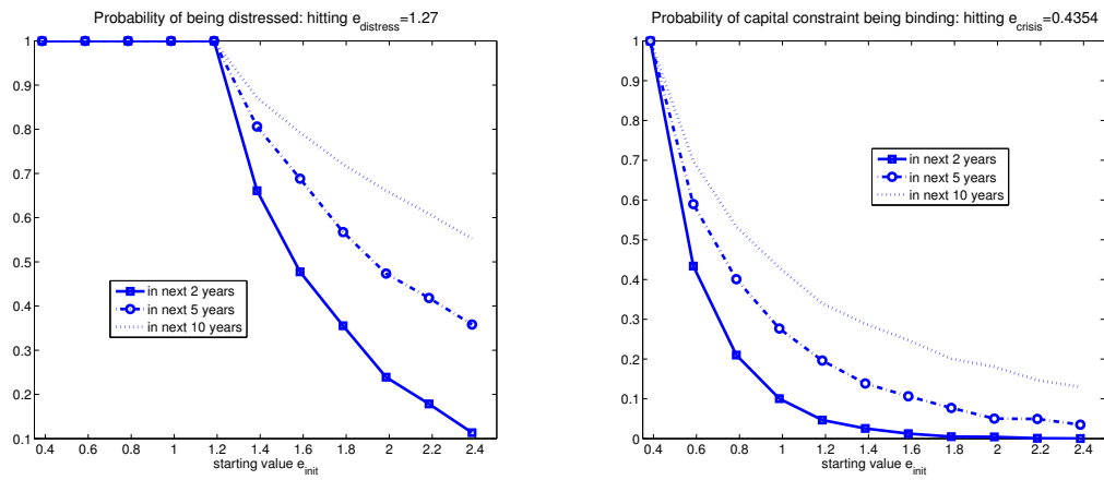
Figure 8: The figure graphs the probabilities of entering distress states (left panel) and states where the capital constraint binds (right panel), anytime over the next 2, 5 and 10 years, conditional on a given value of the state variable e .
