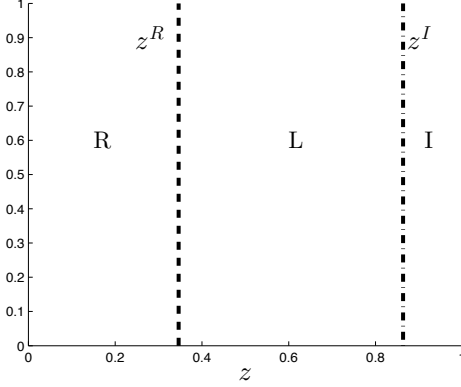
Figure 2: Equilibrium Regions
