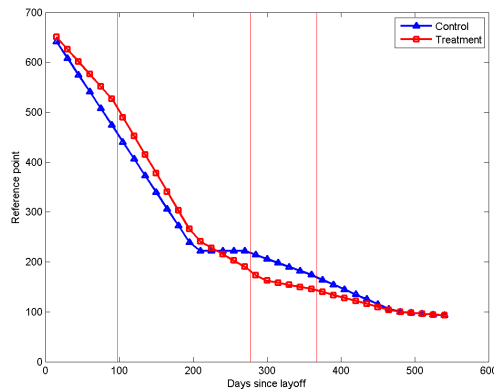
(e) Reference Point, Reference-Dependent Model
