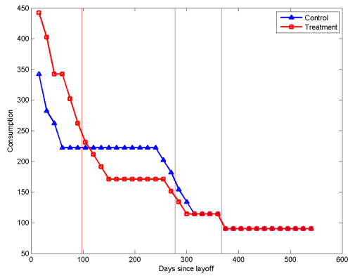
(c) Consumption, Standard Model
