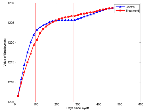
(b) Value of Employment, Reference-Dependent model
