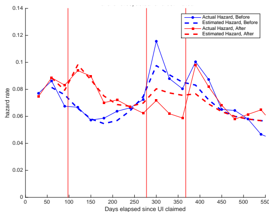
(b) Ref. Dep. Model: 30 Day Hazards
