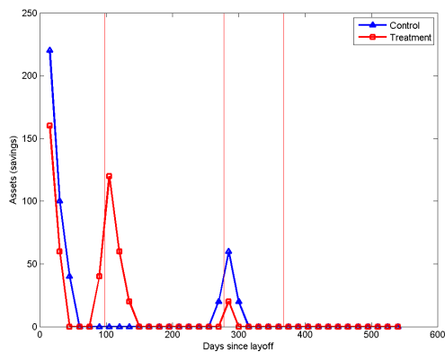
(e) Assets, Standard Model
