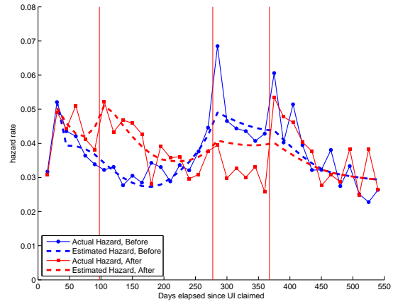
(b) Reference-Dependent Model, no gain
