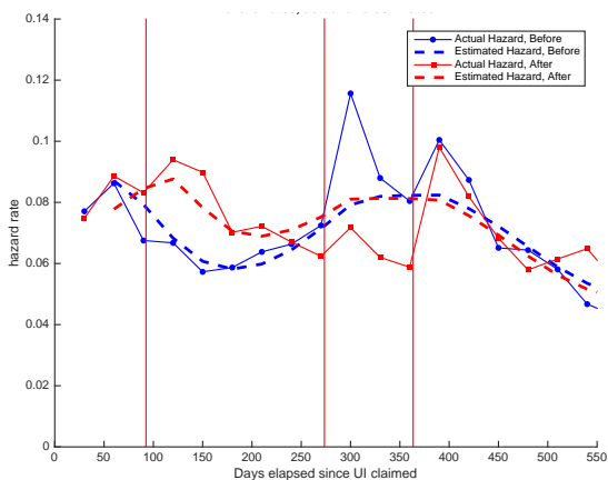
(a) Std. Model: 30 Day Hazards
