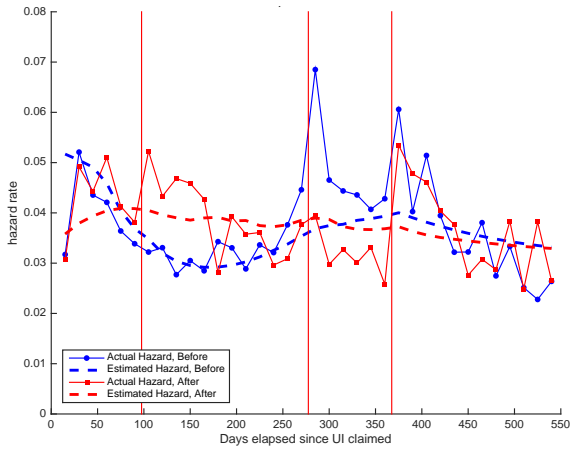
(a) Habit Model with 2 types
