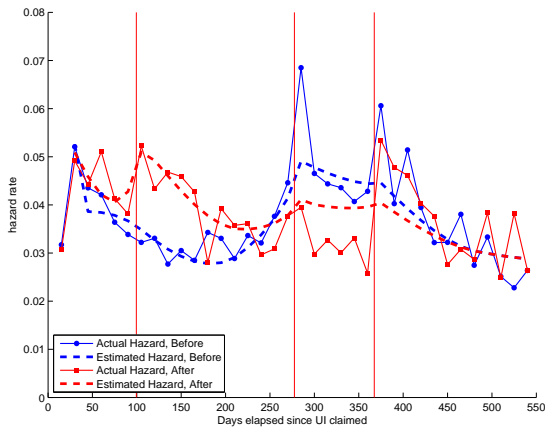
(c) Ref. Dep. Model, 2 cost types, estimated \beta
