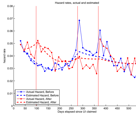
(b) Hazard rate in Ref. Dep. Model
