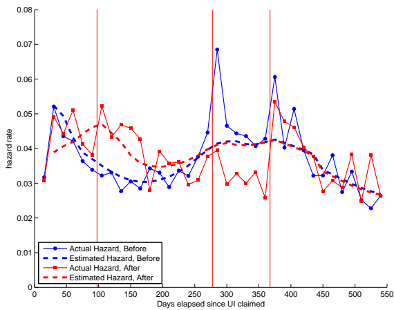
(c) Habit Model with 3 types
