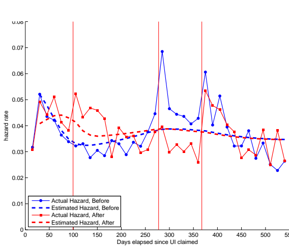
(c) Heterogeneity in Wages
