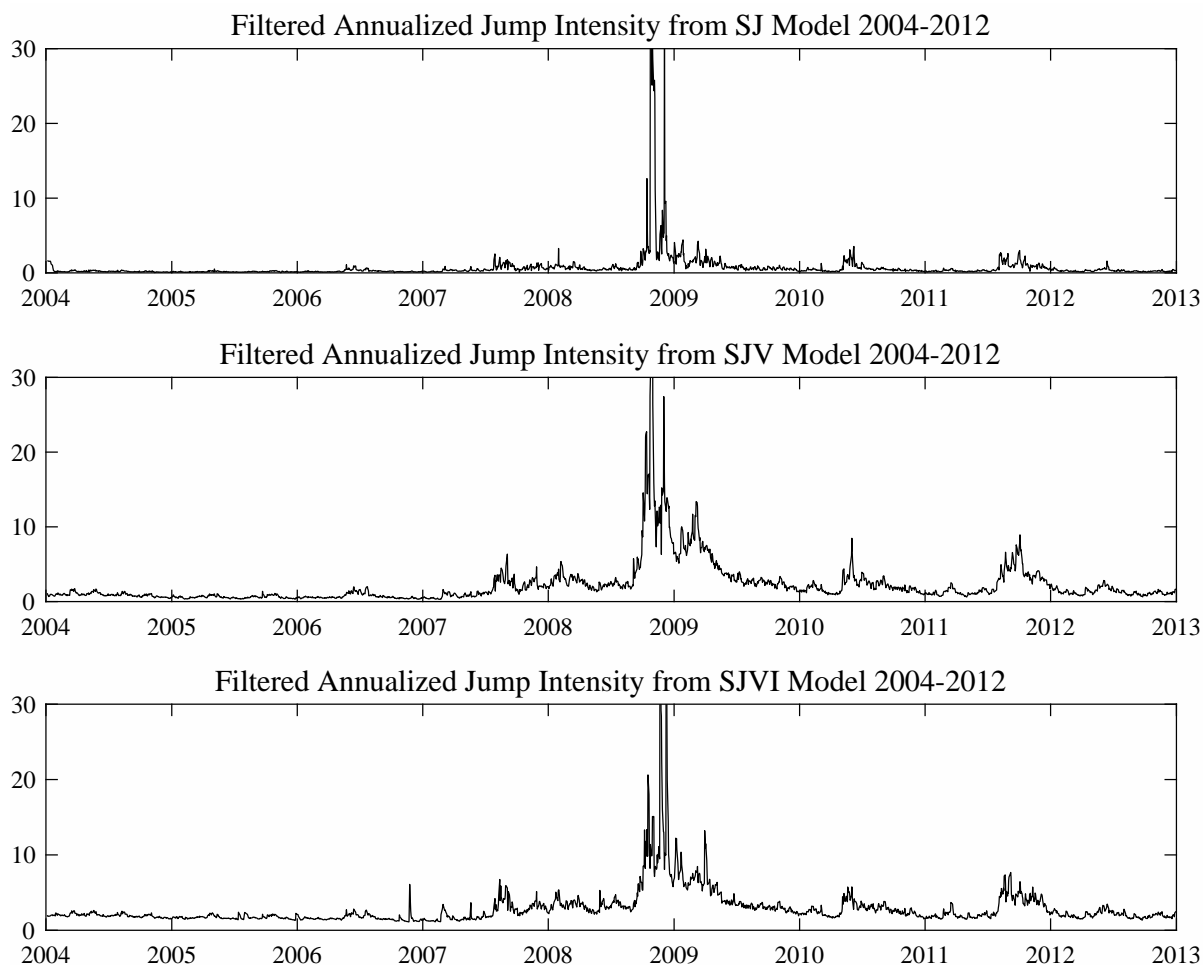
Figure 3: Filtered Jump Intensity: \lambda_t
