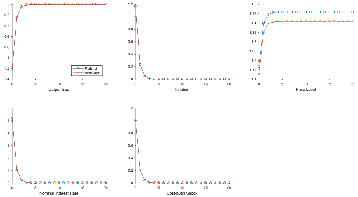
Figure 4: This figure shows the optimal interest rate policy in response to a cost-push shock ( \nu_t ), when the central bank follows the optimal discretionary strategy. The behavior is very similar in the two cases, as the central bank does not rely on future commitments for its optimal policy. This illustrates Proposition 4.4.
