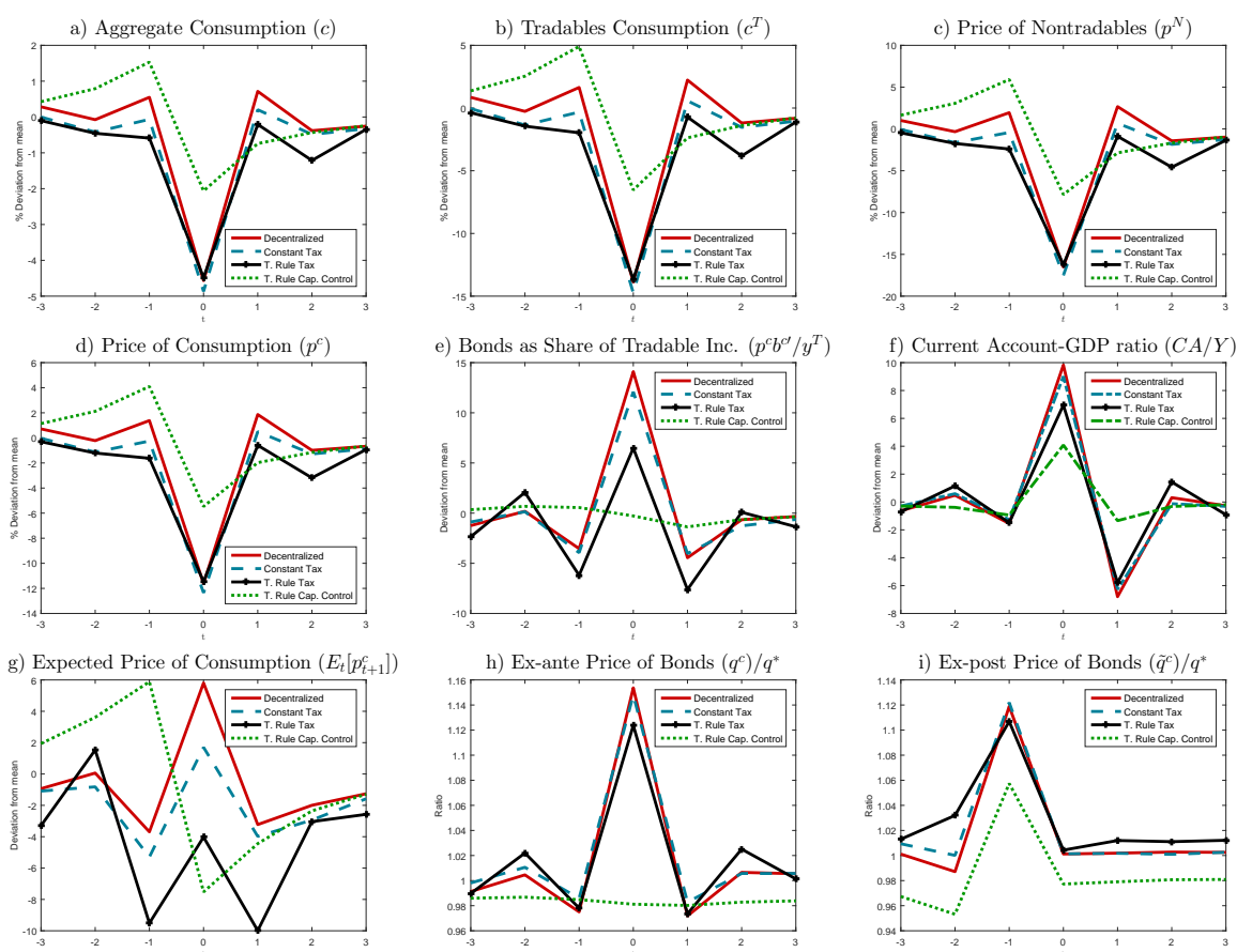
Figure 8: Sudden Stop Events: Unregulated Economy v. Regimes with Simple Policies
