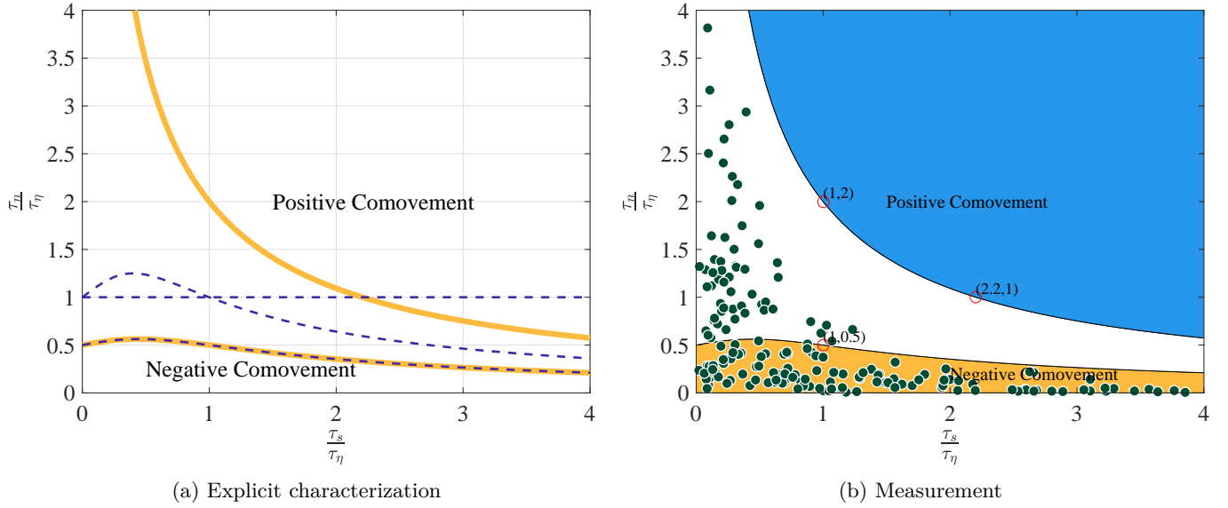
Figure 6: Comovement regions
