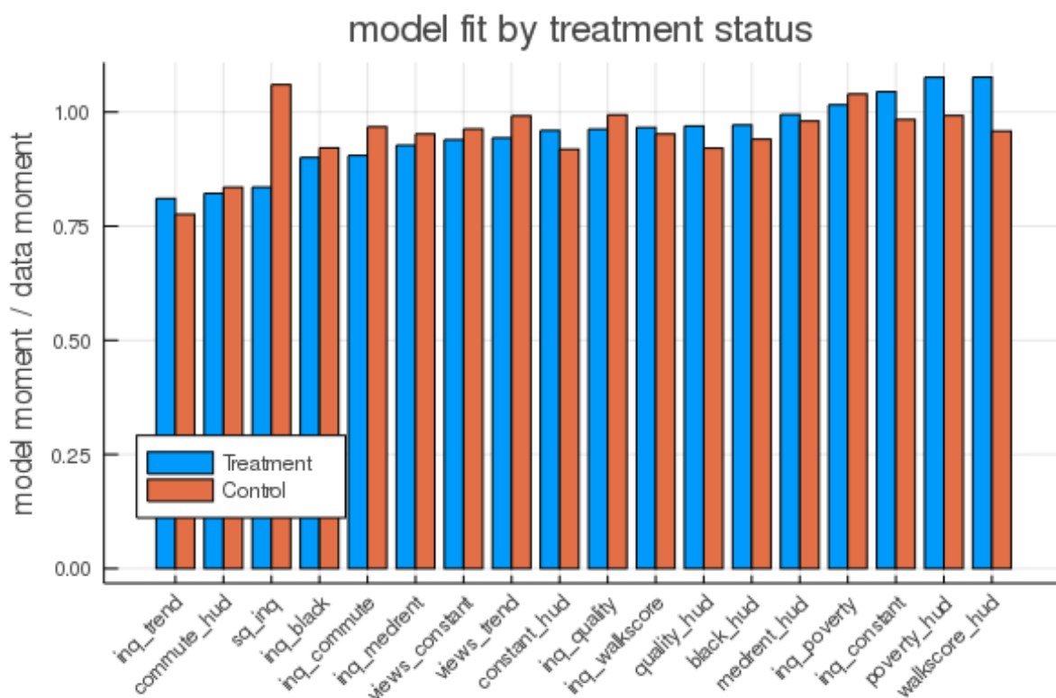
Figure 14: Model fit: all moments
